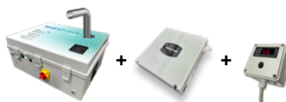
Model HAF-C 500 12 Dimensions: 500x400x190mm For cold rooms up to 500m 3
