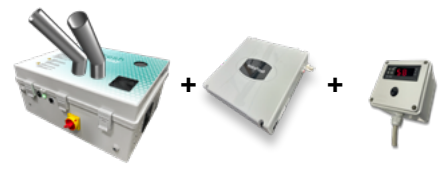
Model HAF-C 1500 24 Dimensions: 600x500x200mm For cold rooms up to 1.500m 3
